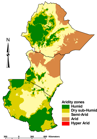
Figure 1. Aridity zones for Eastern Africa
